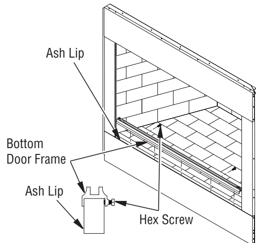
Figure 30 - Installing Bottom Door Frame
