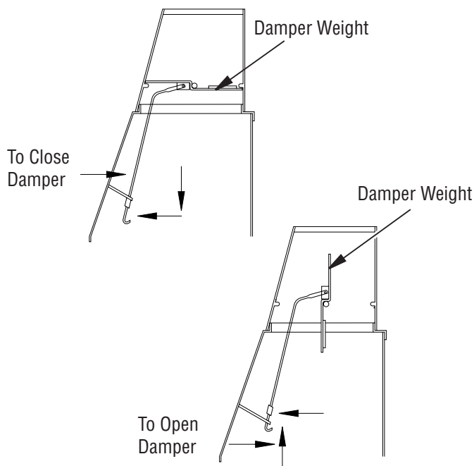
Figure 34 - Operating Damper Handle
