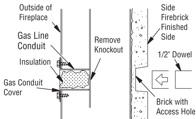
Figure 27 - Gas Line Access
