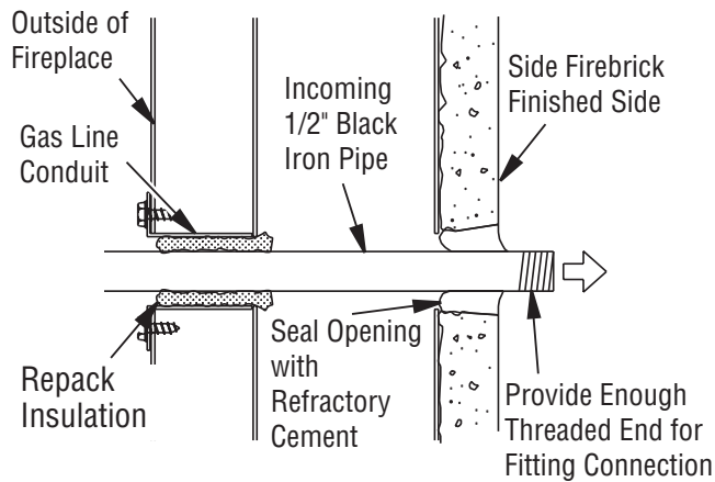
Figure 28 - Gas Line Installation
