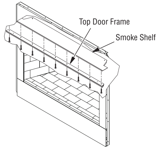
Figure 29 - Installing Top Door Frame
