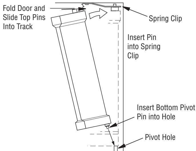
Figure 31 - Installing Bi-Fold Doors
