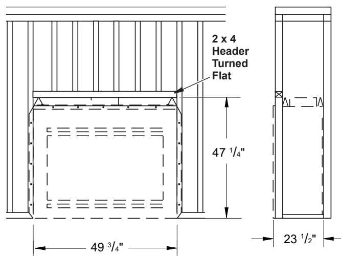
Figure 1 - Framing Dimensions
