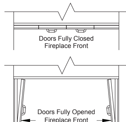
Figure 24 - Glass Doors
