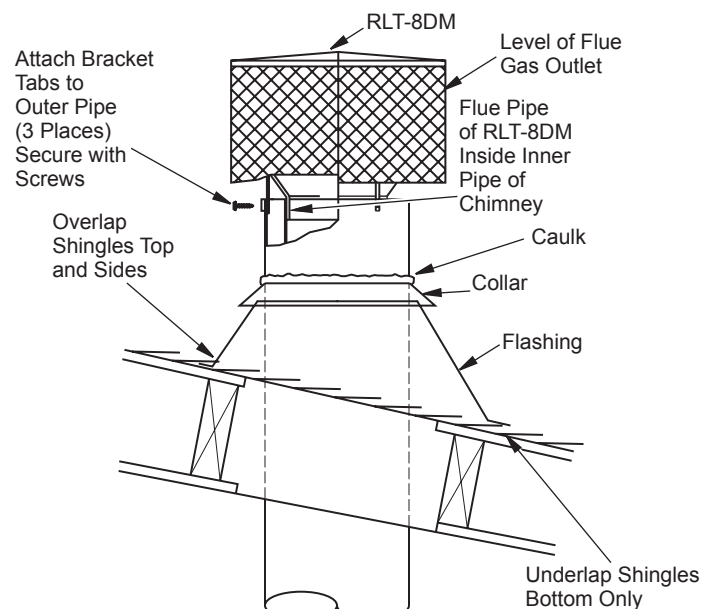
Figure 18 - Termination
