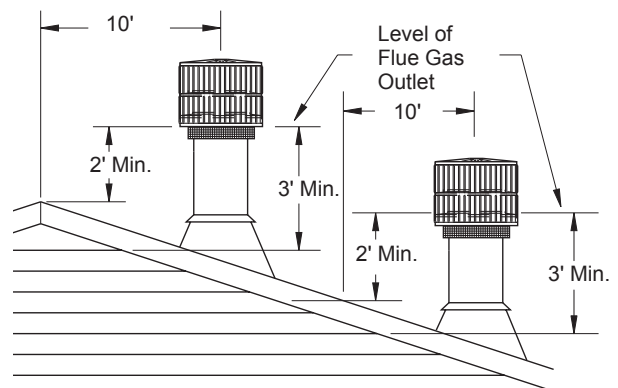
Figure 20 - 10 Foot Rule
