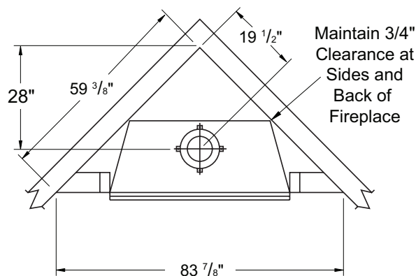
Figure 1 - Framing Dimensions
