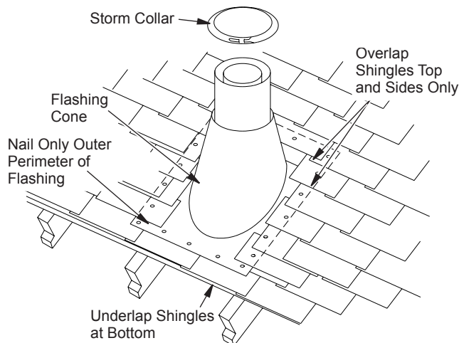
Figure 16 - Flashing Installation
