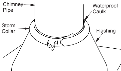
Figure 17 - Storm Collar
