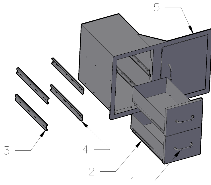
ISOMETRIC VIEW WITH ITEM#'S
