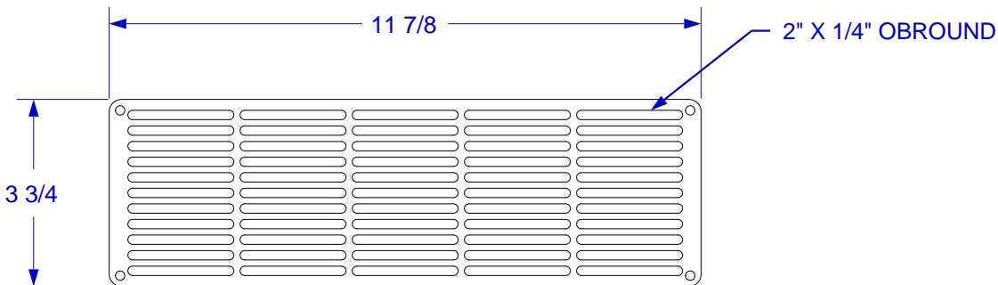
FRONT VIEW
