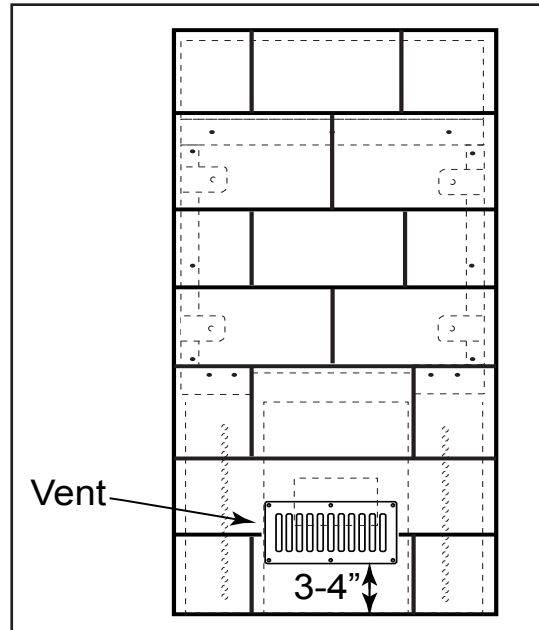
Fig. 3B Vent location.
