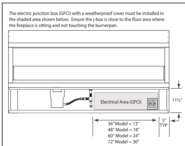
Fig. 13 Electrical placement.
