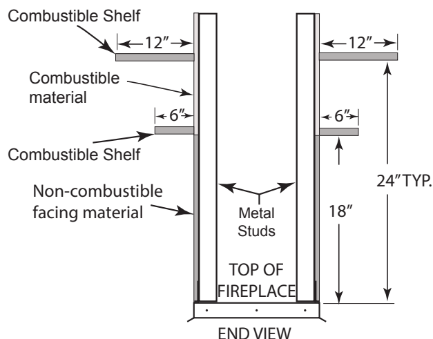
Fig. 11 See-through fireplace mantel clearances
