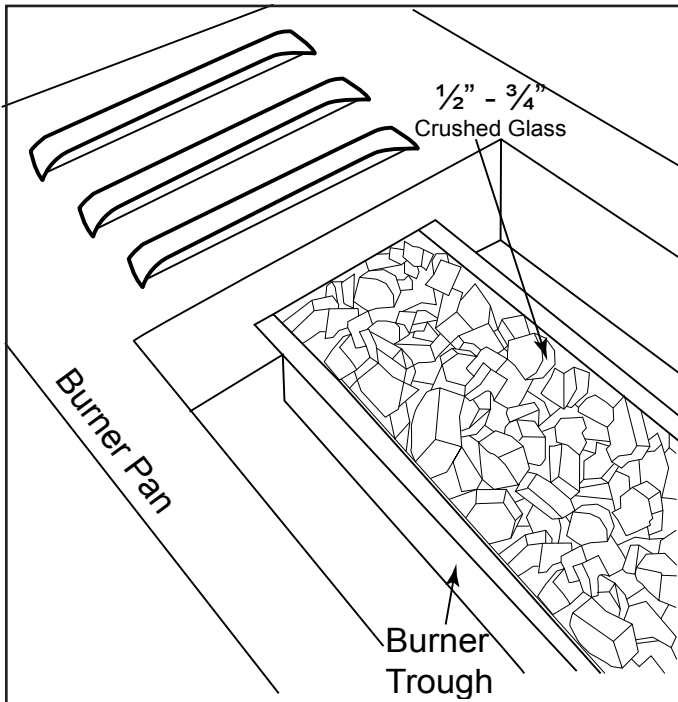
Fig. 34 Installing media into the fireplace.
