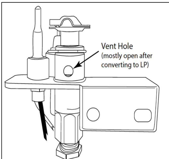
Fig. 9 Pilot assembly converted to LP
