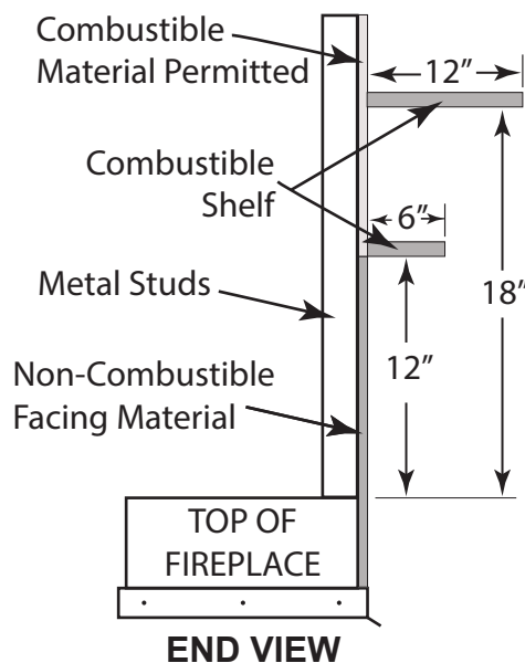
Fig. 7 Open front fireplace mantel clearances
