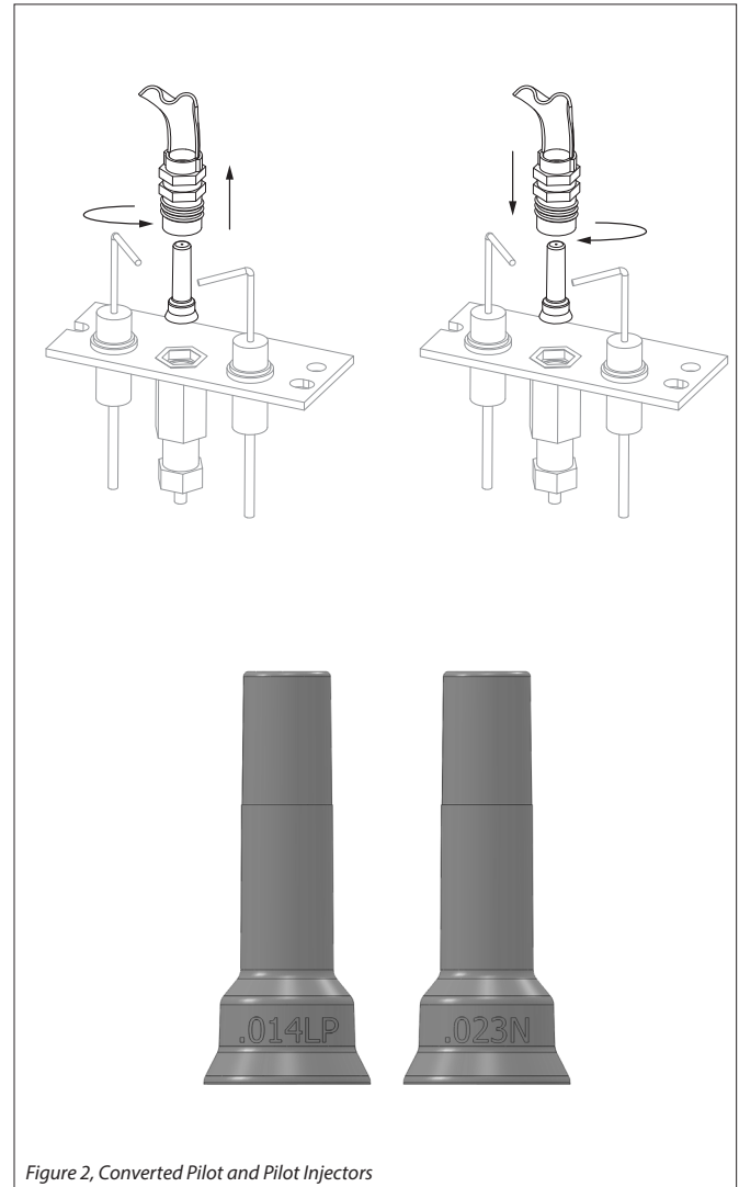
Figure 2, Converted Pilot and Pilot Injectors
