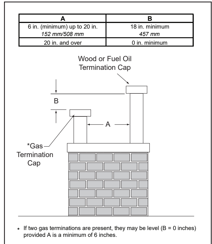
Figure 4.2 Staggered Termination Caps
