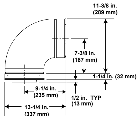
DVP90ST (90° Elbow)
