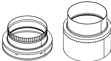
DVP-2SL Adapter
