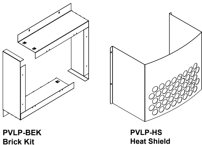
Figure 12.8 PVLP-SLP Vent Components
