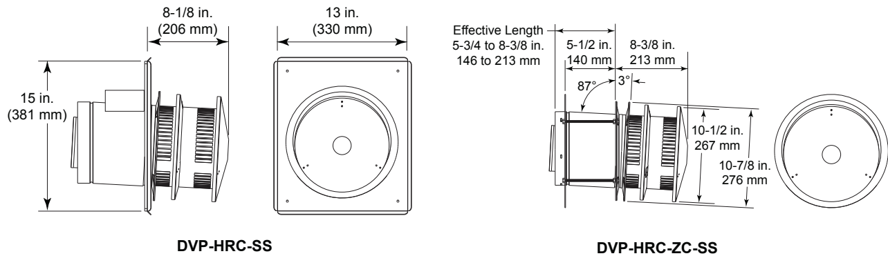
Figure 12.5 Vent Components
