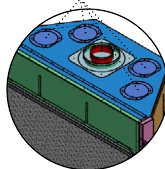
Venting ports (shown on a DRSQ46)
