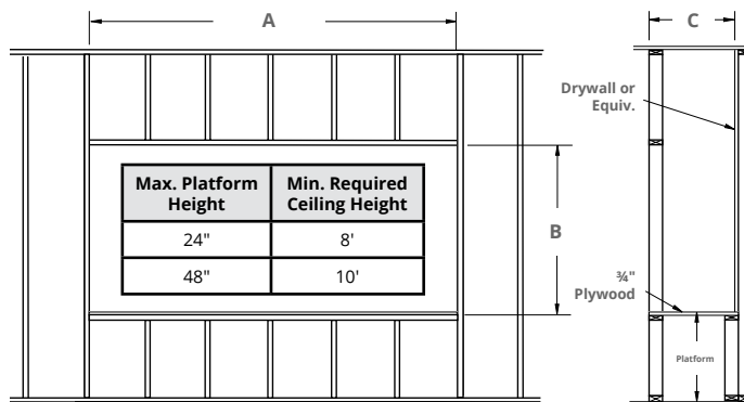
Figure 3.f Fireplace installation, (Rough Frame-In dimensions).
