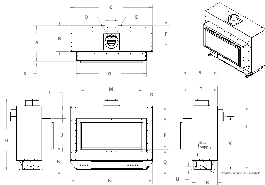
Figure 2. Fireplace dimensions (Tolerance \pm \frac{1}{8} ").
