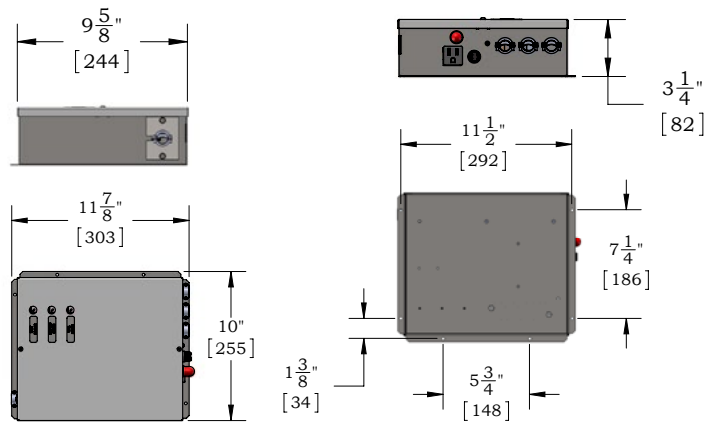
Figure 2.b Control Box Dimensions (Tolerance \pm \frac{1}{8} ").
