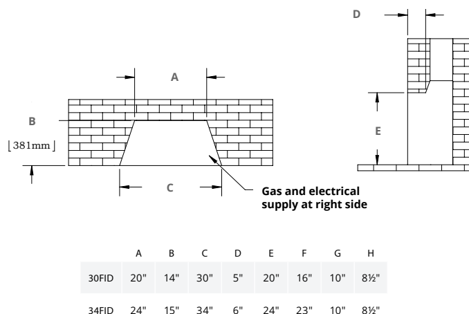
Figure 2.0 Install dimensions
