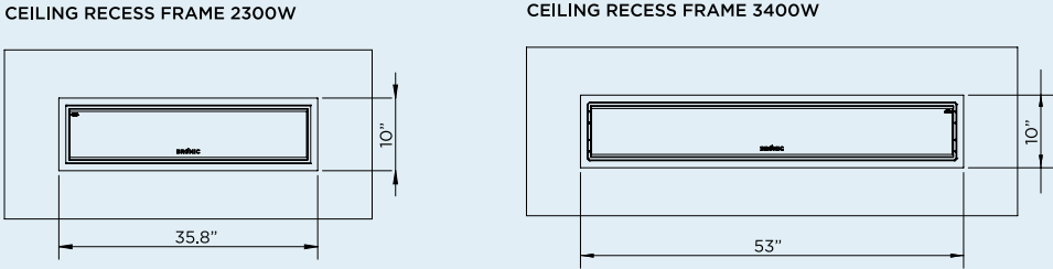
OPTION 1 - STANDARD CAVITY SPACE
