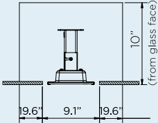
OPTION 1 - STANDARD CAVITY SPACE
