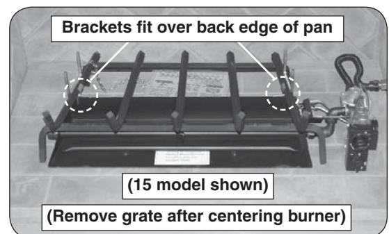
Fig. 17-3 Position grate
