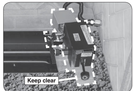
Fig. 18-3 Proper lava media placement
