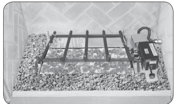
Fig. 20-3 Place grate
