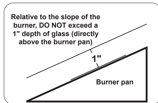
Fig. 13-2 Proper media placement
