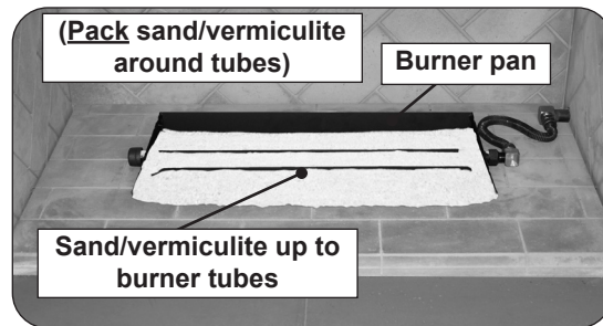
Fig. 12-1 Place sand/vermiculite
