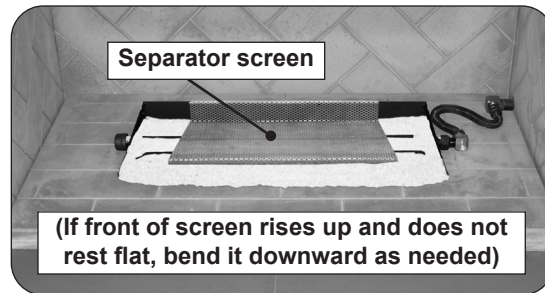
Fig. 12-2 Place screen
