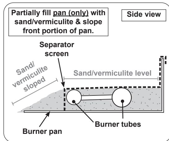
Fig. 12-3 Sand/vermiculite & screen detail
