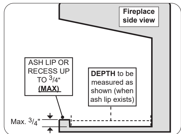
Fig. 6-1 Ash lip/recess detail
