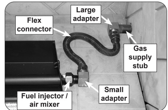
Fig. 11-1 Connect gas supply
