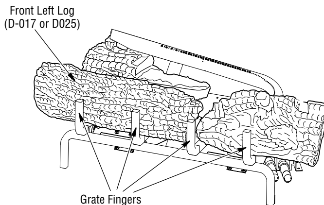
Figure 20 - Installing Front Left Log
