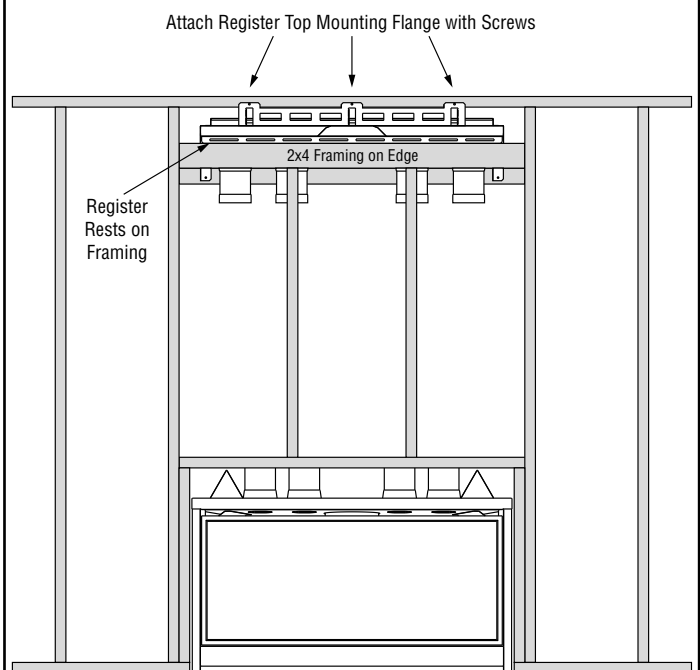
Figure 10 - Securing Register Front View
