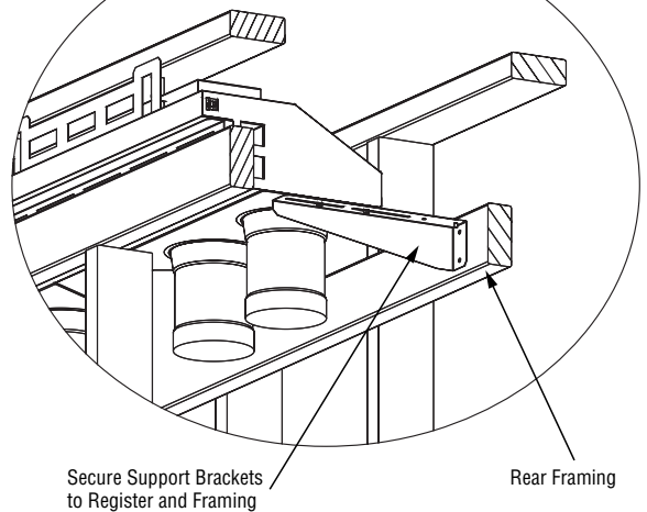
Figure 9 - Installing Support Brackets
