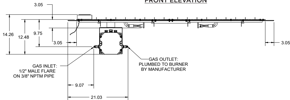
FRONT ELEVATION
