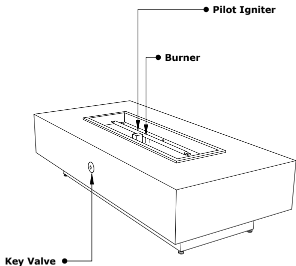
ISOMETRIC VIEW
