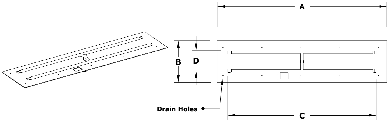
ISOMETRIC VIEW
